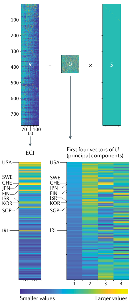
Specialization matrix (sorted by diversity ( M_j ))
