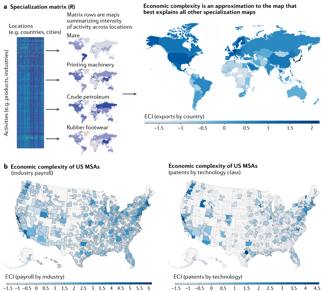
Fig. 2 | Economic complexity. Map of the economic complexity index (ECI) estimated using international trade data (panel a), as well as maps for the ECI of metropolitan statistical areas (MSAs) in the United States estimated using payroll by industry and patents by technology (panel b).
