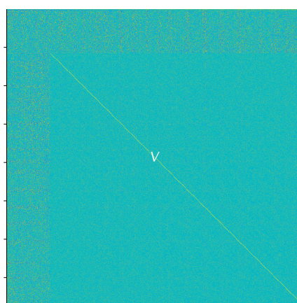
Singular value decomposition
