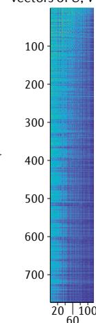
Modelled matrix (using only the first four vectors of U , V and S )
