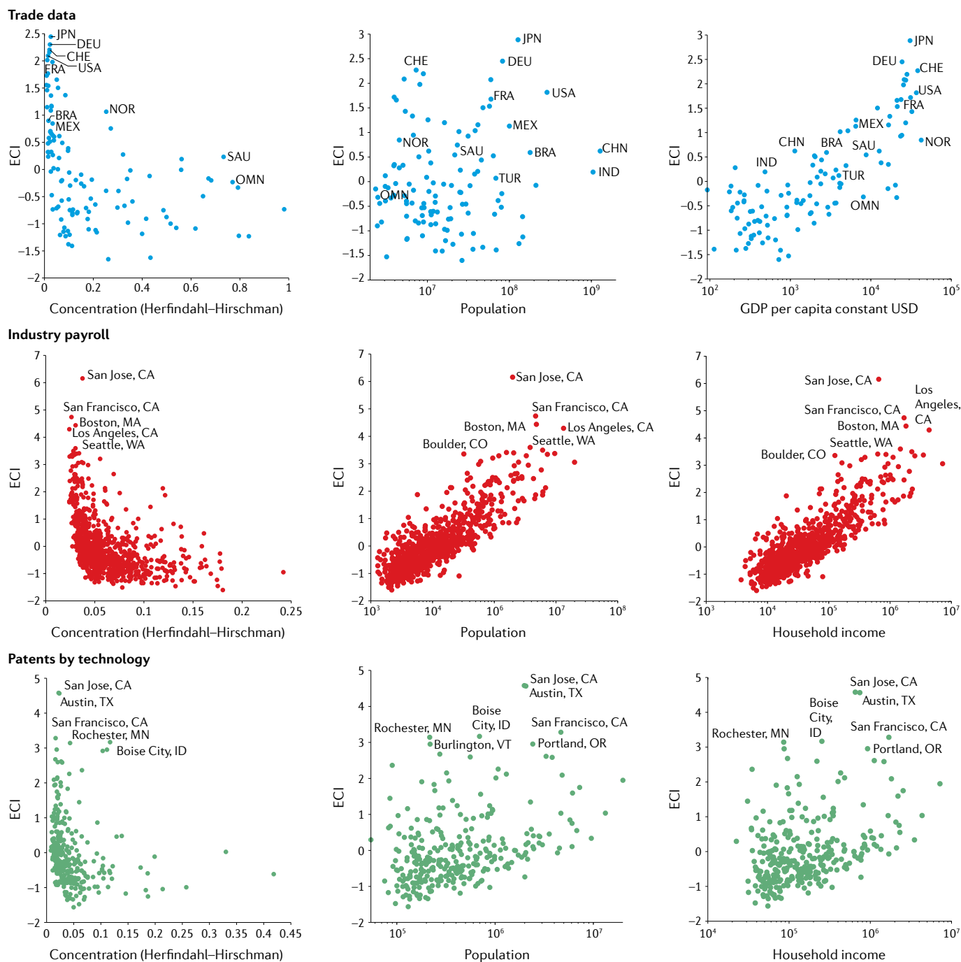
Fig. 4 | Economic complexity compared with measures of concentration, population and income. The economic complexity index (ECI) is computed for regions and US metropolitan statistical areas using trade data, payroll by industry, and patents by technology. GDP, gross domestic product.
