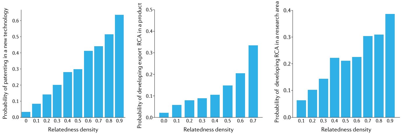
Fig. 5 | Examples of the principle of relatedness in action. The principle of relatedness states that the probability that a location will enter (or exit) an economy activity increases (or decreases) with the presence of related activities in that location. The examples use data from technologies, product exports and research areas 15 . RCA, revealed comparative advantage. Reprinted with permission from REF. 8 , Springer Nature Limited.
